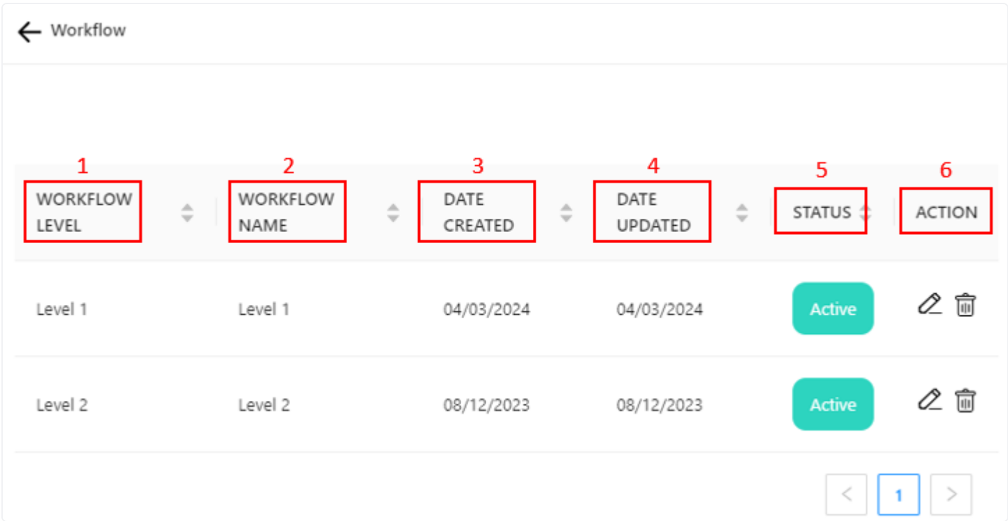
Figure 2.4: More Setting
