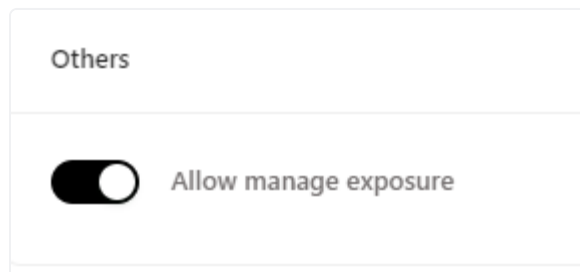
Figure 2.10: Others
