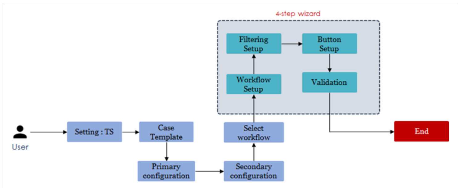
Figure 2.1: Case Template
