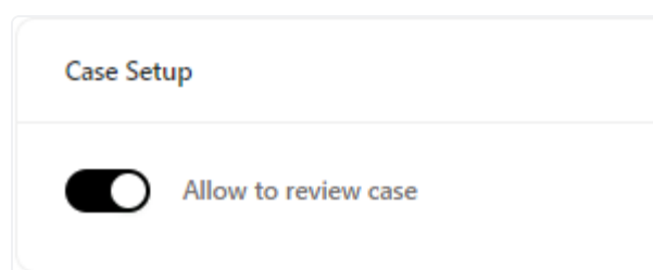
Figure 2.8 Case Setup
