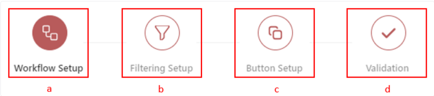
Figure 2.5: 4-Step Wizard
