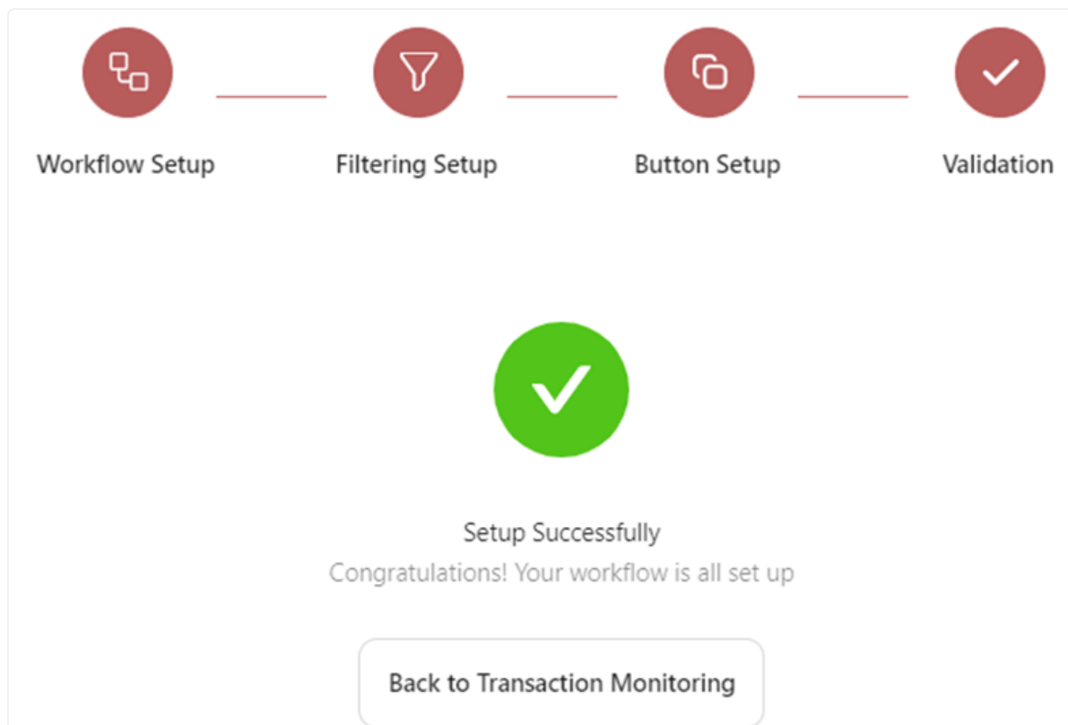
Figure 2.13: Validation
